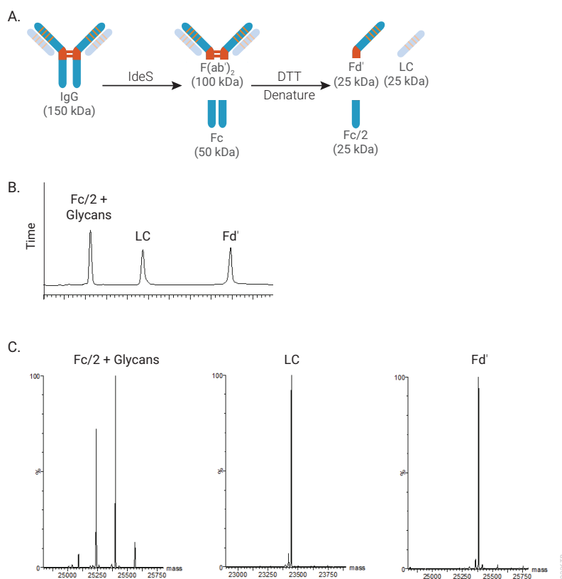
Figure 23. Digestion with IdeS followed by reduction and denaturing produces fragments that are better separated by HPLC and are ideal for mass spectrometry analysis. Panel A: Digestion of IgG with IdeS, followed by reduction, produces three 25 kDa fragments. Panel B: Example of IdeS digestion products separated on HPLC. Panel C: Mass spectrometry results of the three IdeS digestion products.
